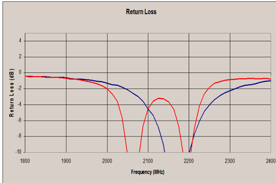
Figure 8. Measured frequency response from prototype null steering antenna
