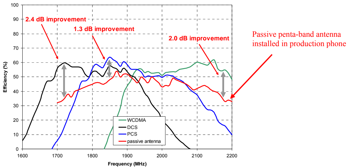
Figure 6. Efficiency of an active, tunable antenna compared to a passive (fixed tuned) main antenna; main antenna is installed in a production handset
