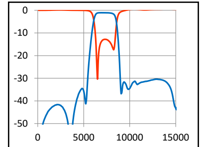
0805 size Central Frequency: 7.25 GHz Passband: 1.25 GHz
