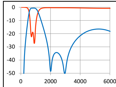
1206 size Central Frequency: 0.8 GHz Passband: 250 MHz
